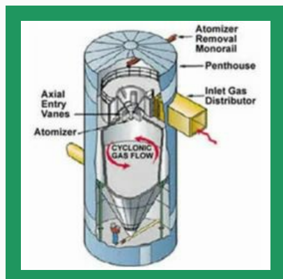
Dry Air Scrubber
